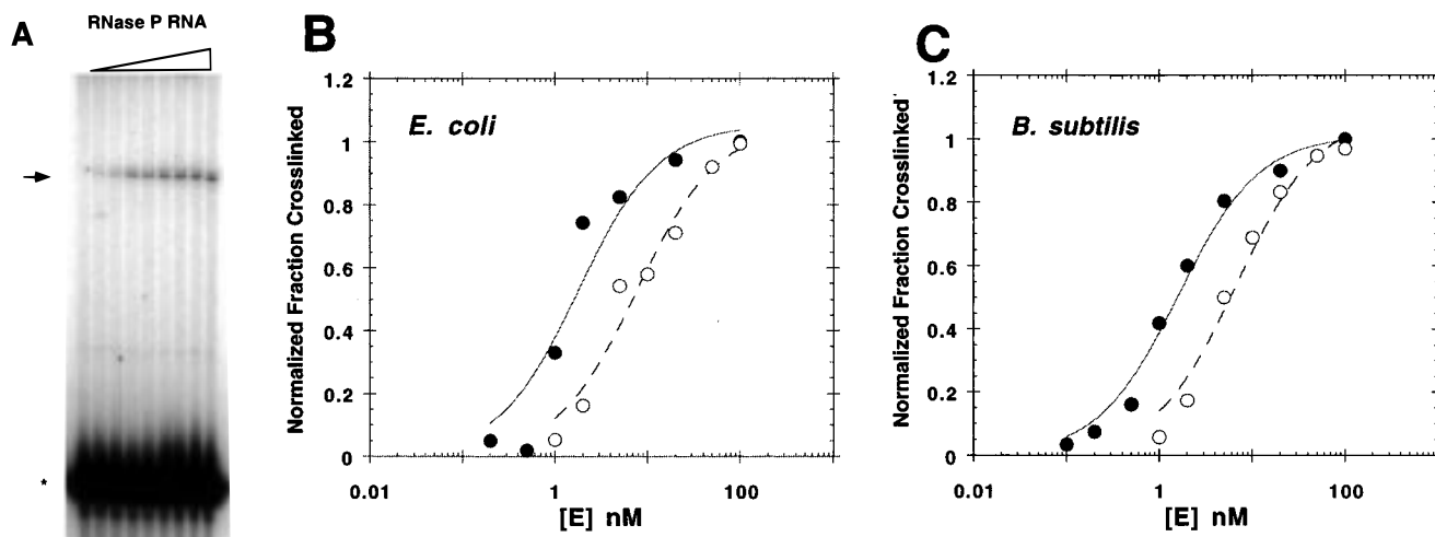
FIGURE 6: Measurement of dissociation constant ( K_{Dapp} ) by cross-linking. 5'- ^{32} P-End-labeled tRNA or tRNA(G-1) containing s ^6 G at their 5' ends were cross-linked to B. subtilis RNase P RNA or E. coli RNase P RNA under buffer conditions described in Figure 4 over a range of enzyme concentrations in which enzyme is kept in excess ( [E]/[S] > 5 with [S] = 0.05 – 2.5 nM). For tRNA, [E] = 0.1 – 100 nM, and for tRNA(G-1), [E] = 1 – 100 nM. (A) Example of tRNA cross-linking to E. coli RNase P RNA. Arrow indicates a position of intermolecular cross-linking; asterisk indicates the position of tRNA. (B, C) Normalized fractions of tRNA (●) or tRNA(G-1) (○) cross-linking plotted versus E. coli RNase P RNA (B) or B. subtilis RNase P RNA (C) concentration. K_{Dapp} was calculated from a fit to eq 1.
